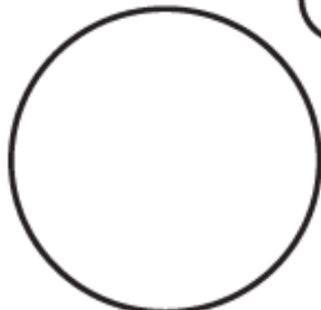
Mercury
