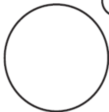
Neptune
